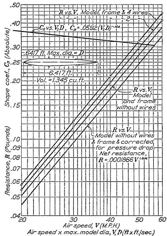
FIG. 12.—Fineness ratio = 10
