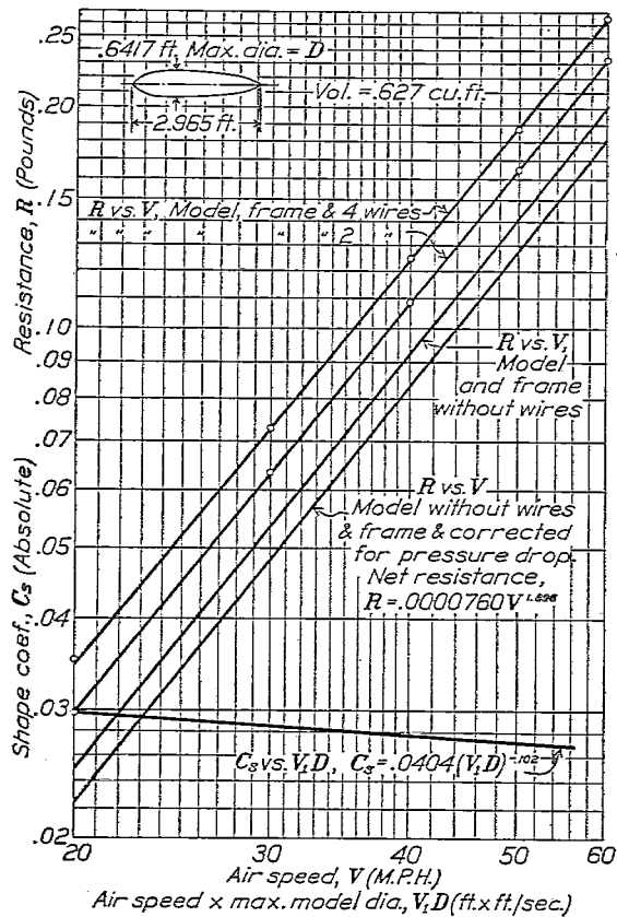
FIG. 9.—Fineness ratio = 4.62
