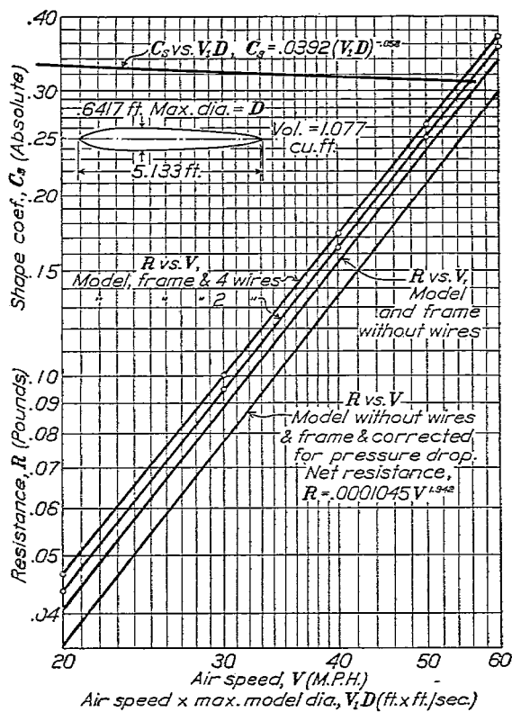
FIG. 11.—Fineness ratio = 8
