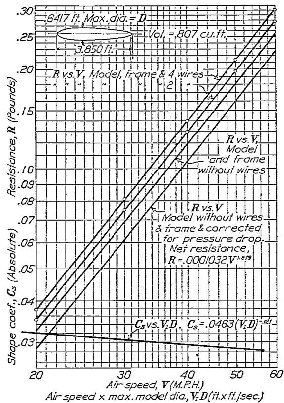
FIG. 10.—Fineness ratio = 6
