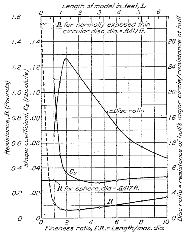
FIG. 13.—C-class airship. Models with various fineness ratios. Air speed 40 M. P. H. Model at 0^\circ pitch and 0^\circ yaw
