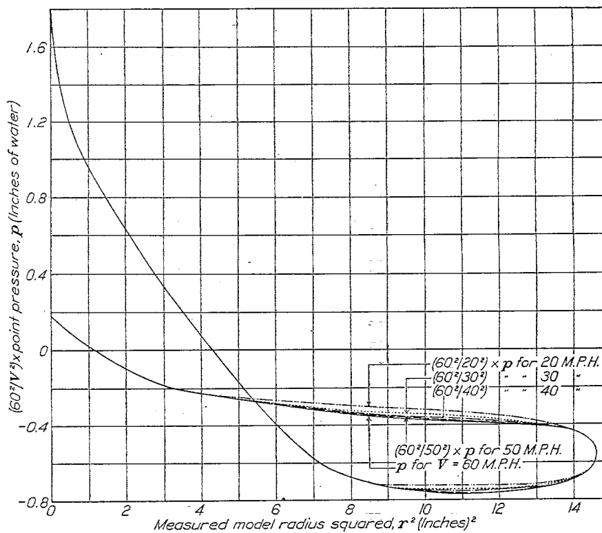
FIG. 16.—C-class airship. Fineness ratio=4.62 Model at 0^\circ pitch and 0^\circ yaw
