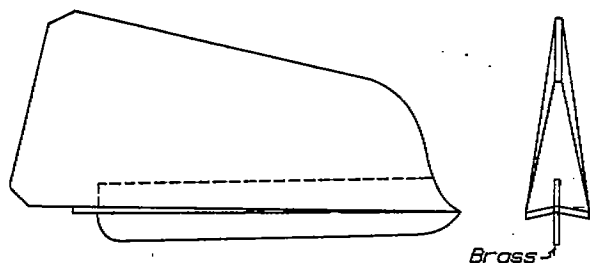
FIGURE 2.—Goodyear-Zeppelin airship models. Wood V fins. The brass fins are made of brass plate. They are of the same general plan form as the wood V fins and are \frac{1}{16} inch thick
