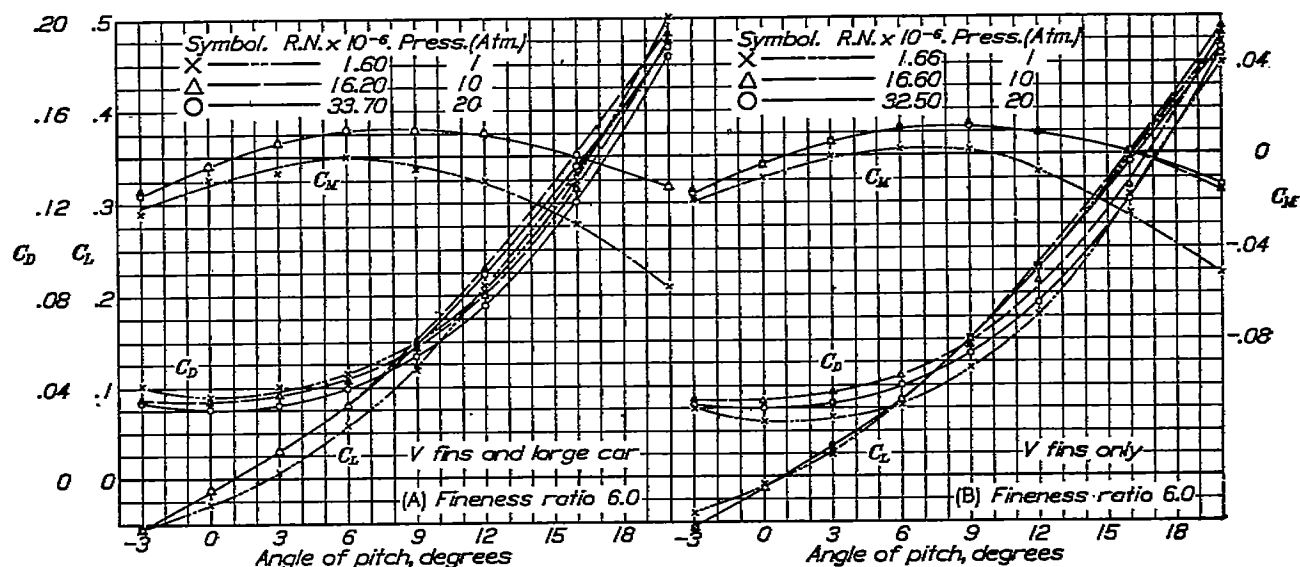
FIGURE 15.—Effect of car on aerodynamic characteristics of the GZ-6.0 model in pitch. Tested in the closed-throat tunnel
