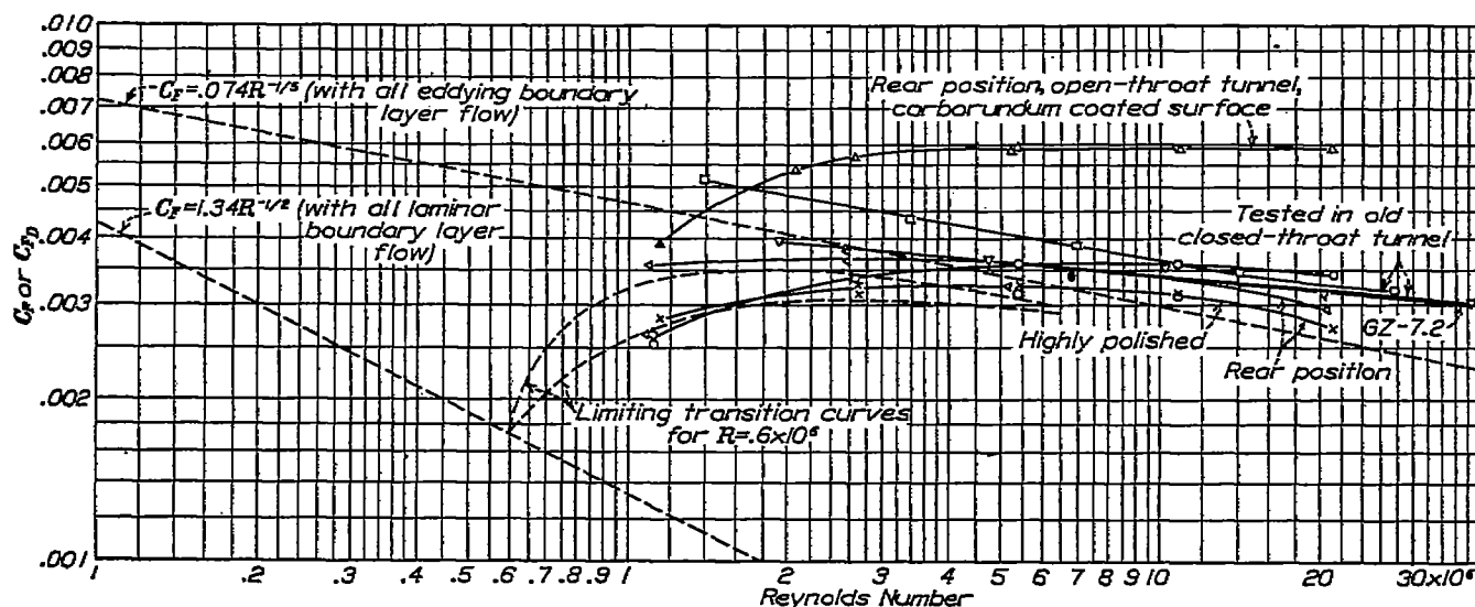
FIGURE 23.—Comparison of skin friction on airship models and rectangular flat plates. Dashed lines represent theoretical curves for skin friction on rectangular flat plates. Solid lines represent test results on bare-hull airship models. These curves are for the GZ-4.8 model tested in the normal position with normal surface in the open-throat tunnel except as noted.
