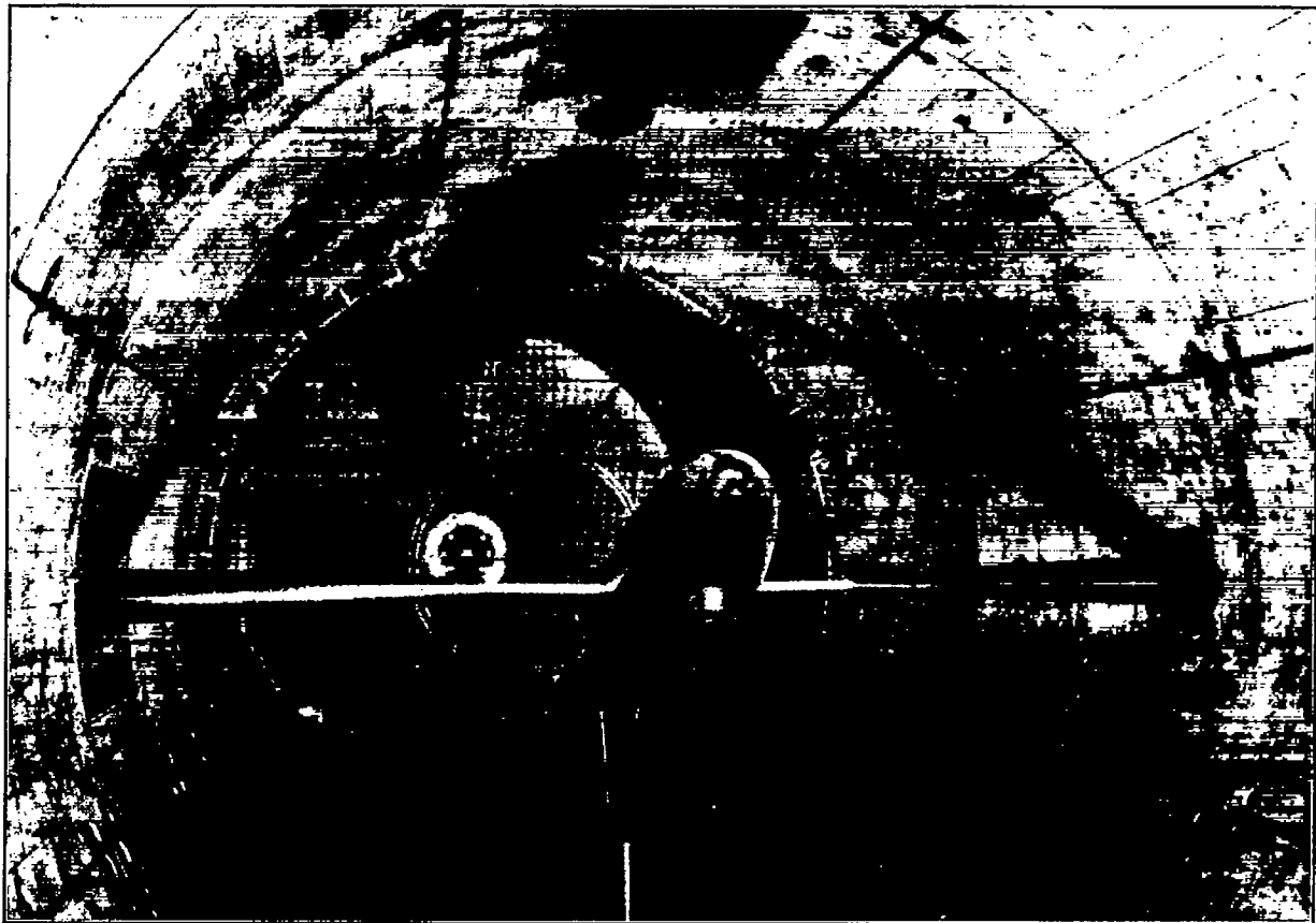
FIGURE 5.—Goodyear-Zeppelin airship model mounted at 20° pitch on the main balance of the closed-throat tunnel
