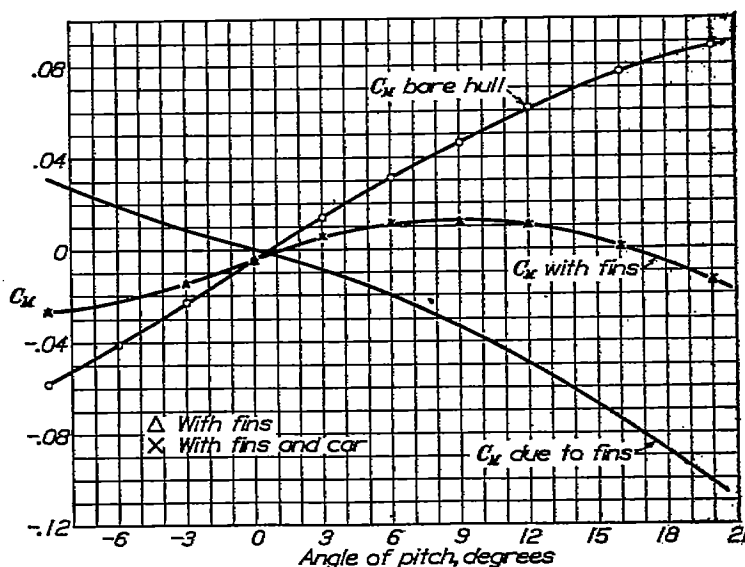
FIGURE 24.—Moment due to fins and fins and car. Goodyear-Zeppelin airship model. Fineness ratio, 6.0; Reynolds Number 33 \times 10^6
