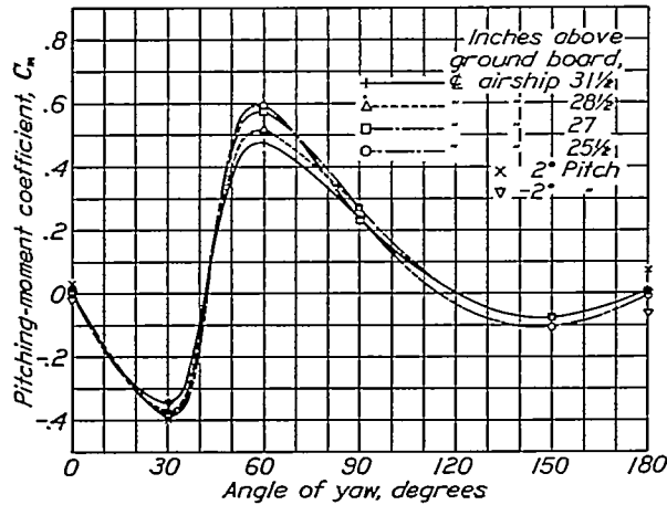
FIGURE 16.—The variation of pitching-moment coefficient with angle of yaw, angle of pitch, and height above the ground board at a Reynolds Number of 16,000,000.
