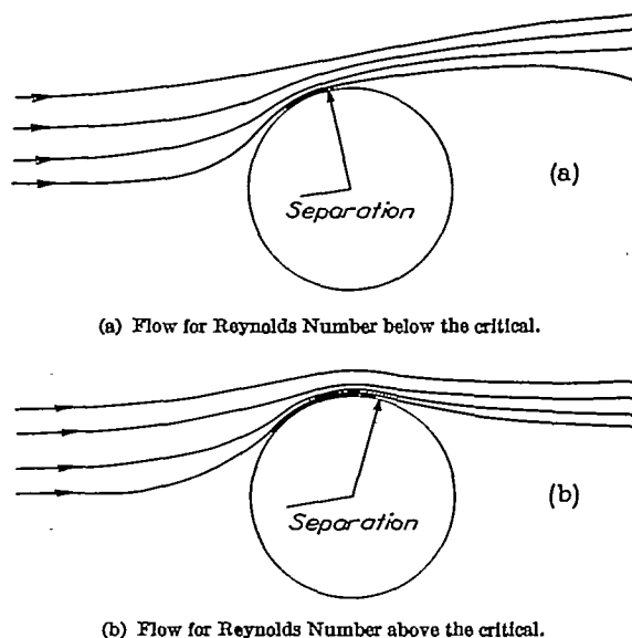
FIGURE 25.—Flow over circular cylinders showing separation.
