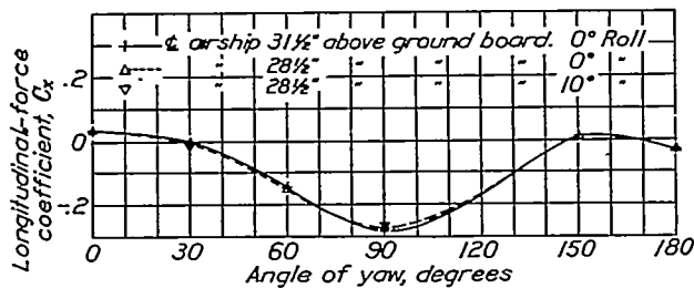
FIGURE 12.—The variation of longitudinal-force coefficient with angle of yaw, angle of roll, and height above the ground board at a Reynolds Number of 8,000,000.
