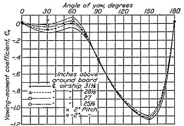
FIGURE 19.—The variation of yawing-moment coefficient with angle of yaw, angle of pitch, and height above the ground board at a Reynolds Number of 16,000,000.
