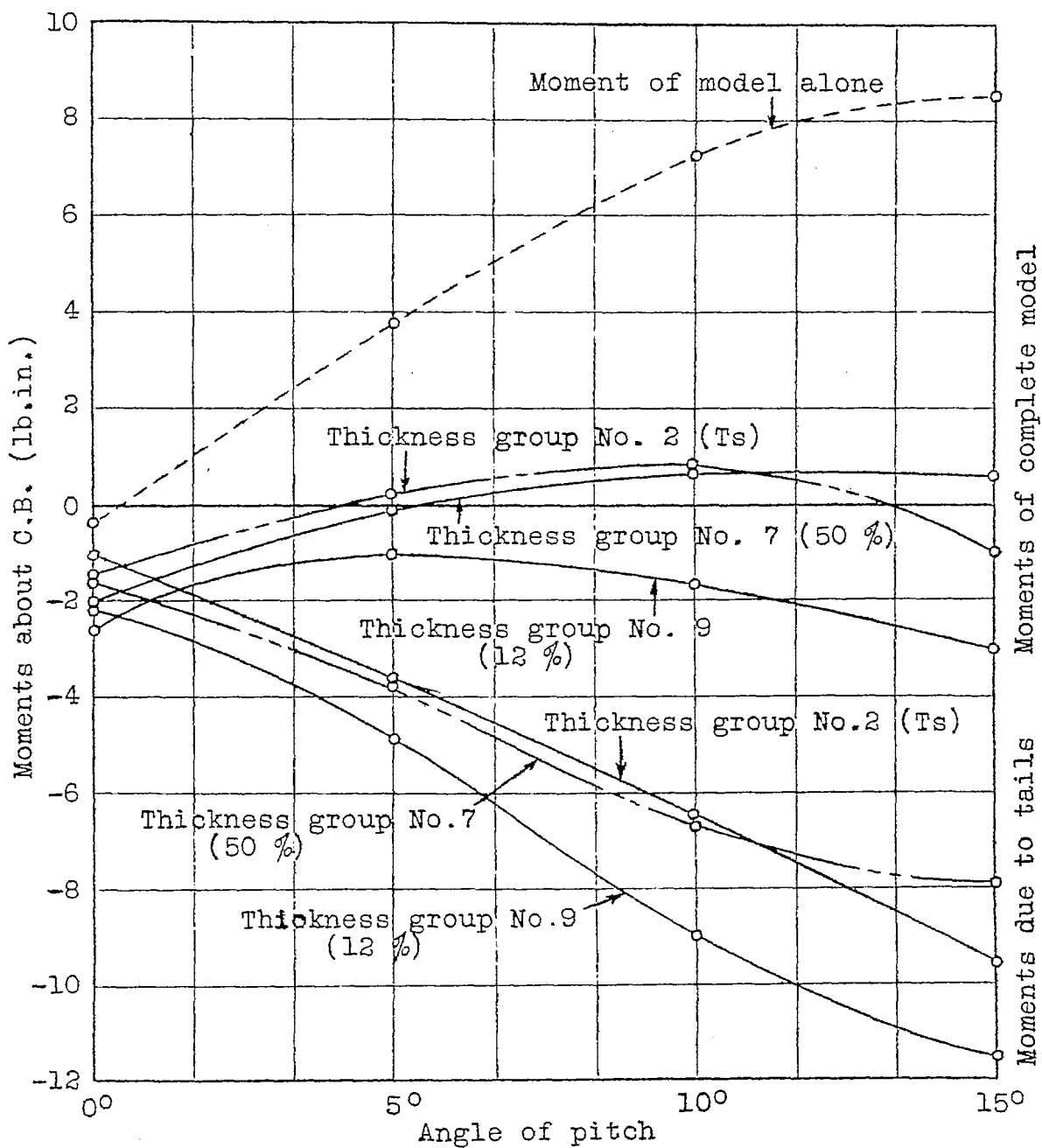
Moment curves for elevator angle 10°
