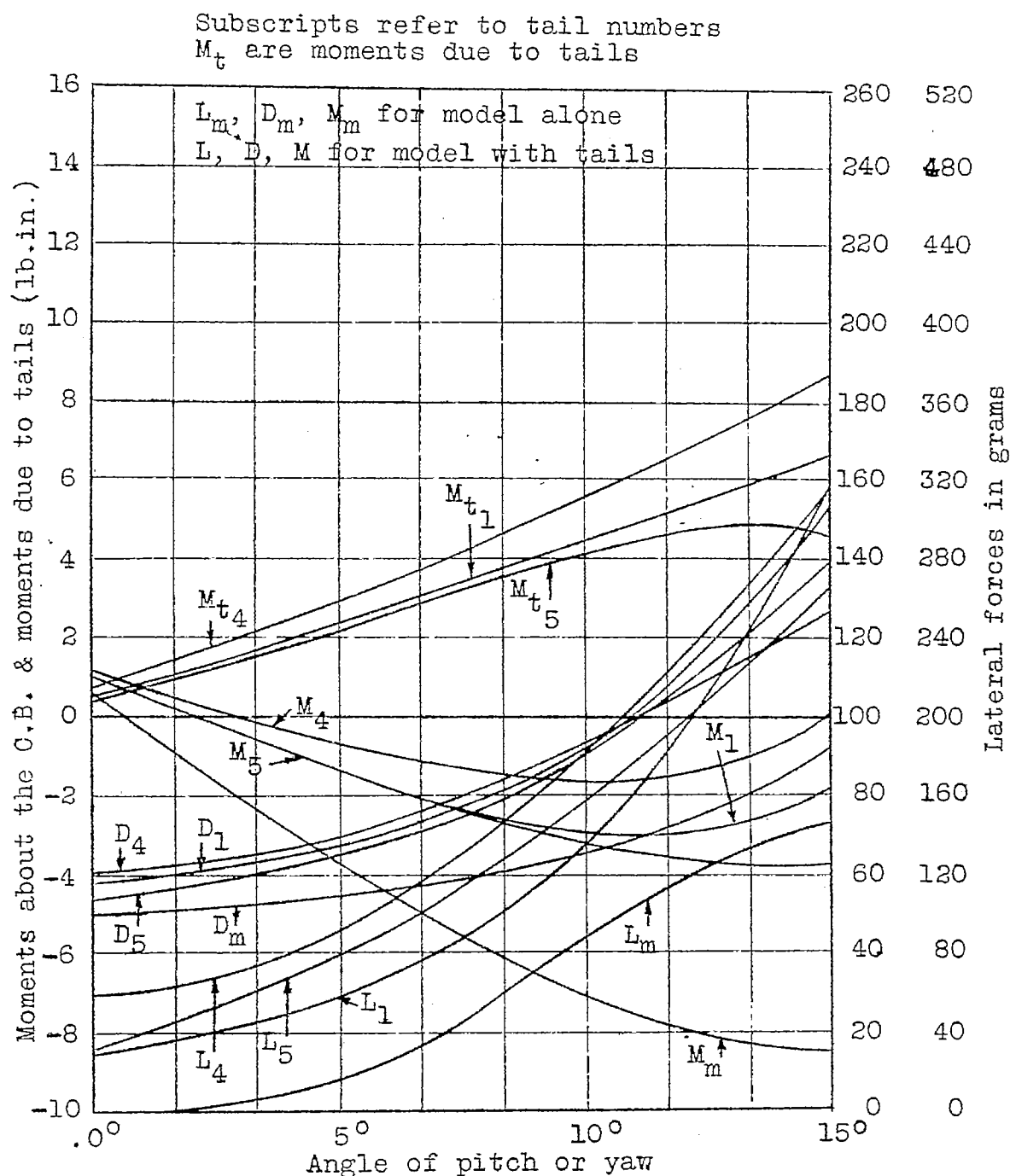
Fig. 17 Performance curves of an L-33 model fitted with aspect ratio tail surfaces. Elevators 10^\circ
