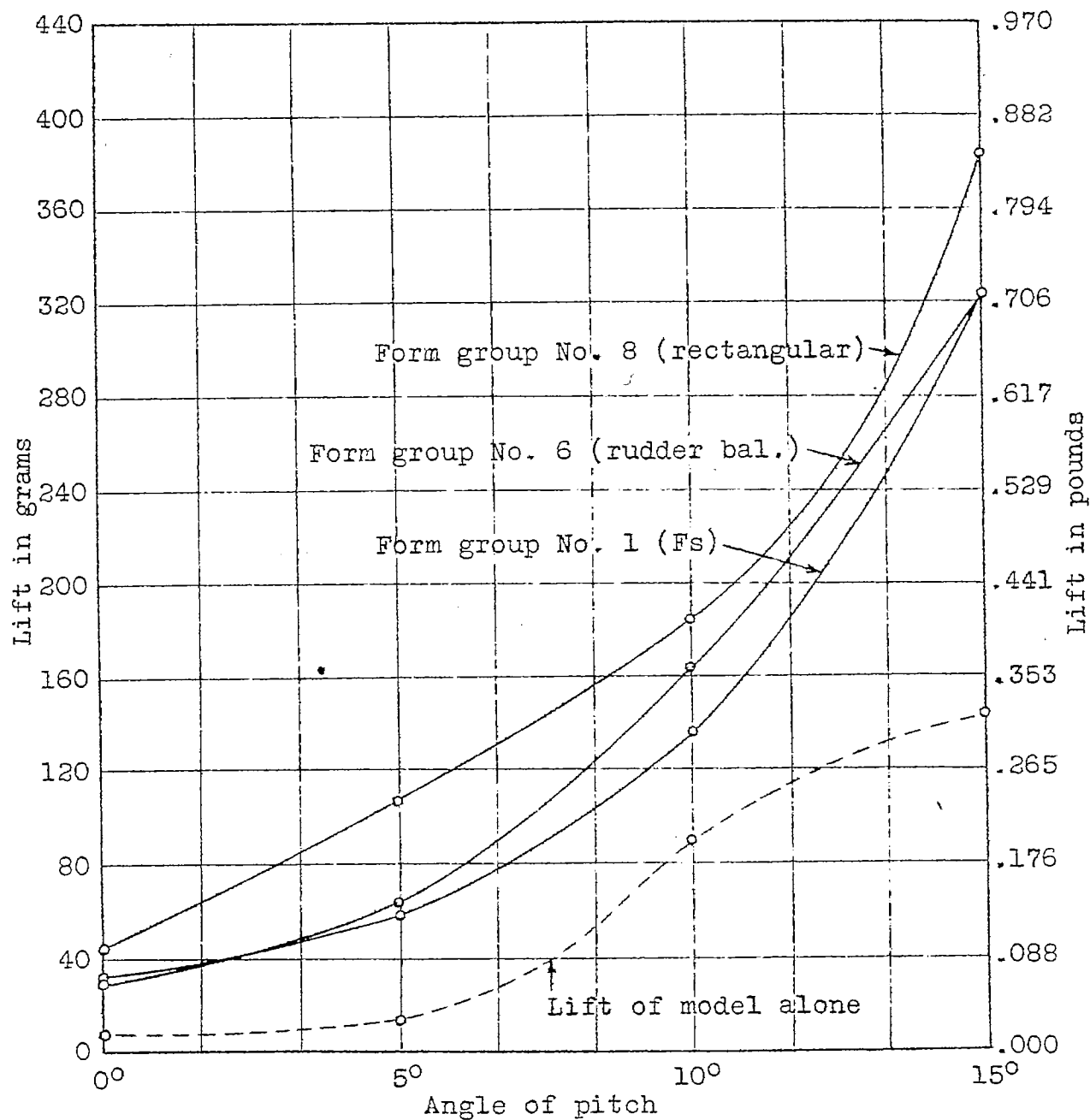
Fig. 7b Lift curves for elevator angle 10°
