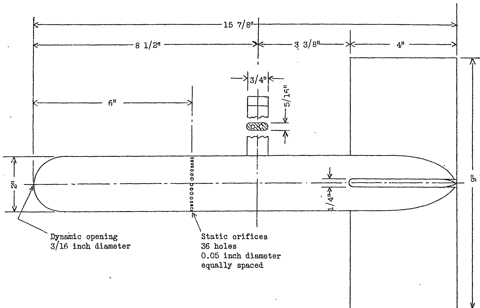
Figure 4.- Suspended air-speed head.
