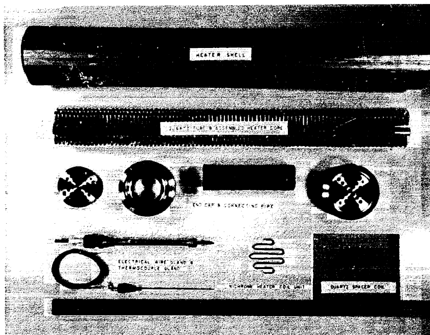
Heater Assembly
