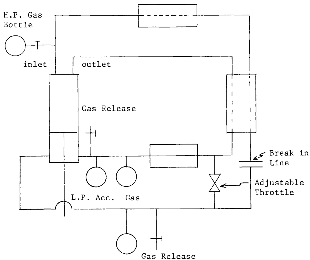
Figure 4. Engine Test Configuration for Experiment 2
