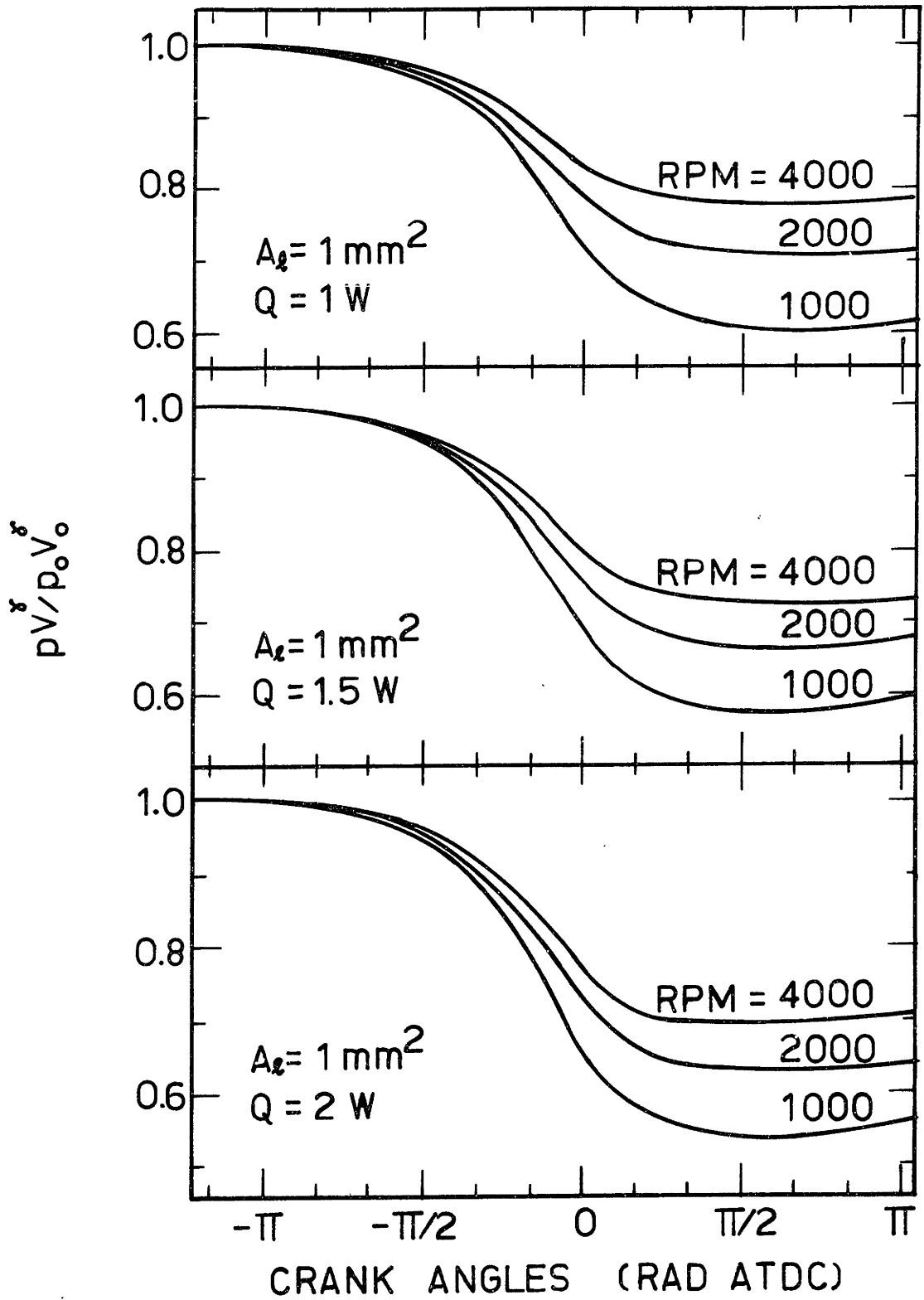
Fig. 26 Change in pV^Y with heat transfer and speed holding constant the leakage.
