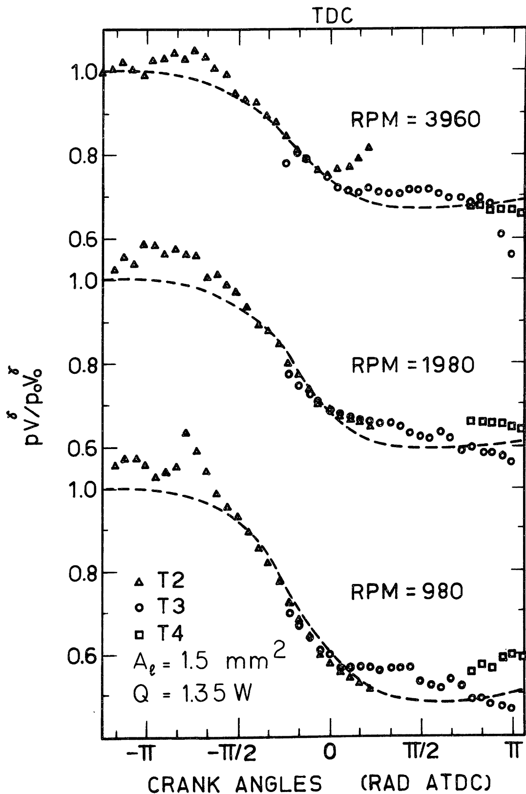
Fig. 21 pV versus crank angle obtained from the various transducers during motoring conditions, versus model predictions (dash).
