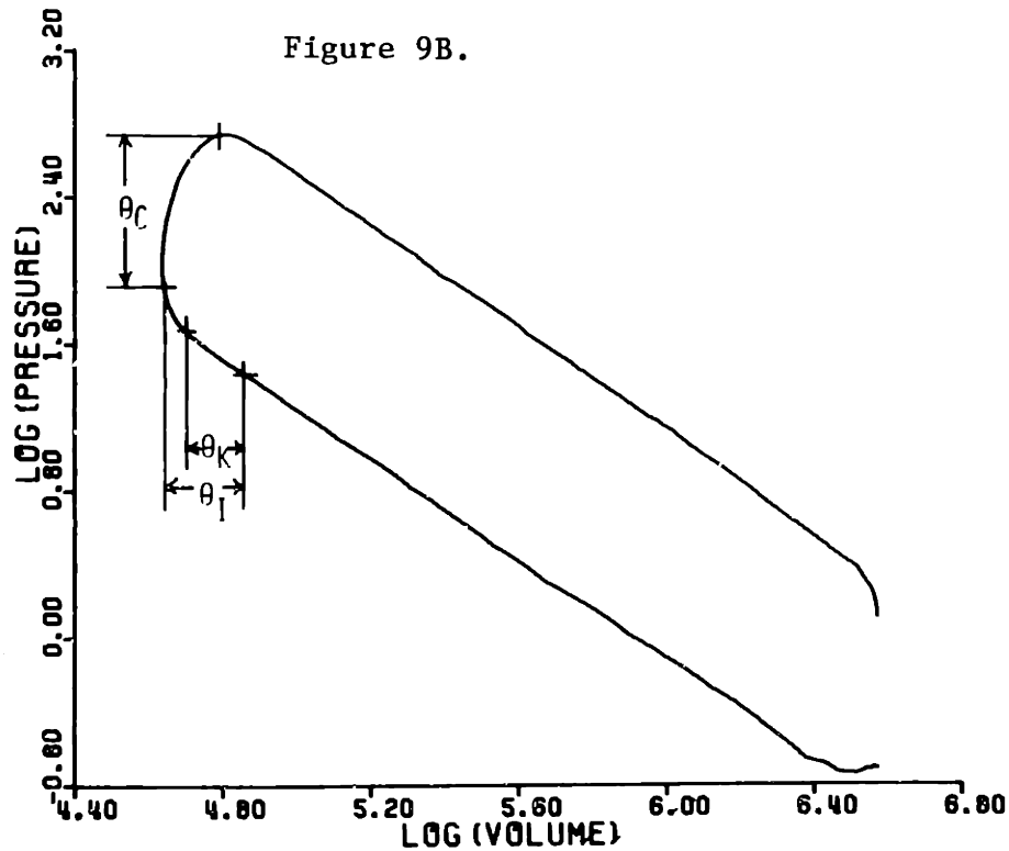
Figure 9 Definitions of kernel development ( \theta_K ), ignition delay ( \theta_I ), and combustion duration intervals ( \theta_C ) on mass fraction burned (x) vs. crank angle ( \theta ) and log (Pressure) vs. log (Volume) diagrams: (9A and 9B) Case #40, \phi = .97 , methanol
