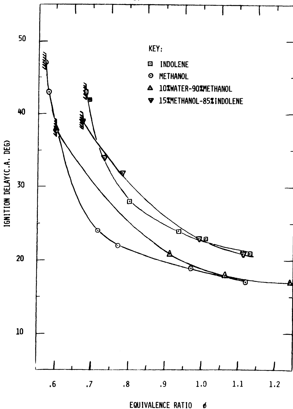
Figure 11 Ignition delay interval ( \theta_I ) vs. equivalence ratio ( \phi ) and fuel type at baseline conditions (Table 4)
