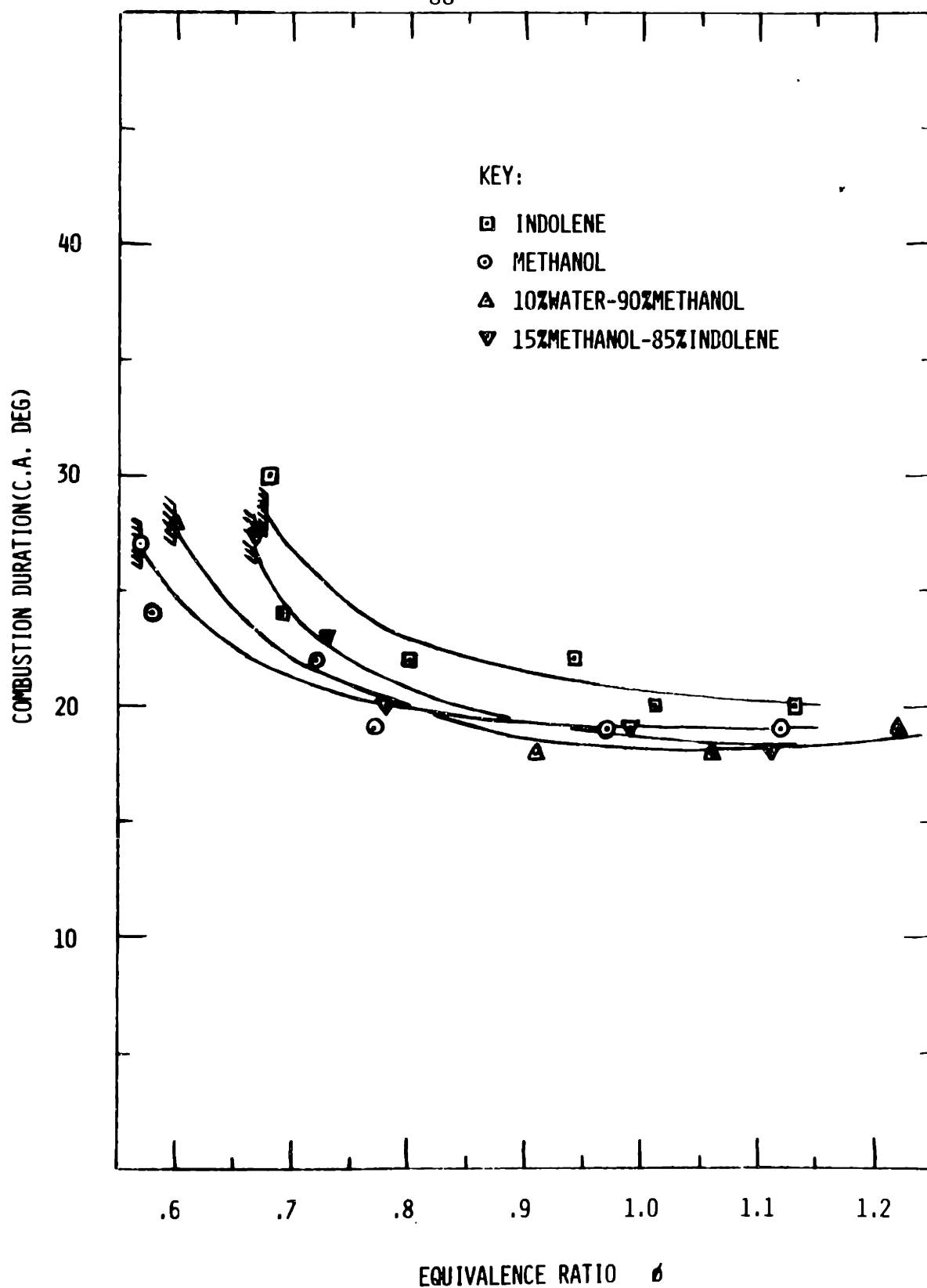
Figure 12 Combustion duration interval ( \theta_c ) vs. equivalence ratio ( \phi ) and fuel type at baseline conditions (Table 4)
