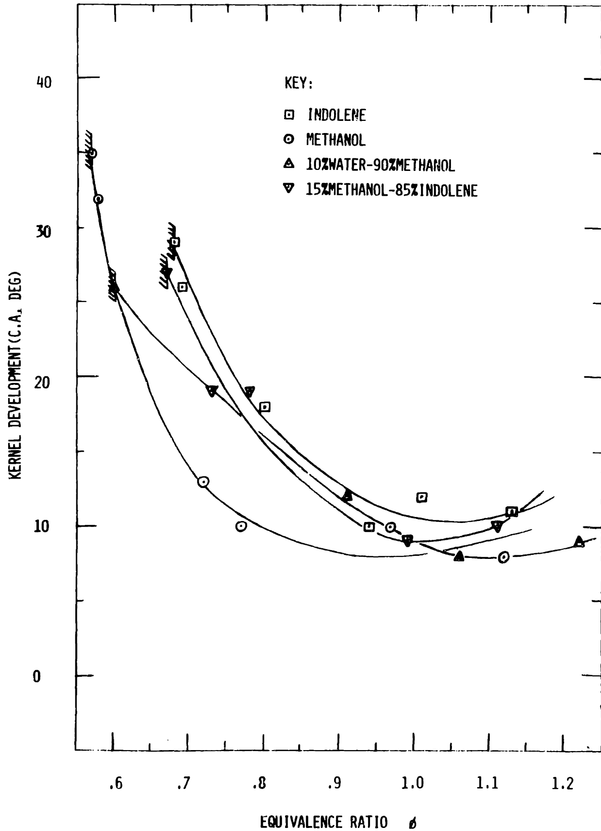
Figure 10 Kernel development interval ( \theta_k ) vs. equivalence ratio ( \phi ) and fuel type at baseline conditions (Table 4)
