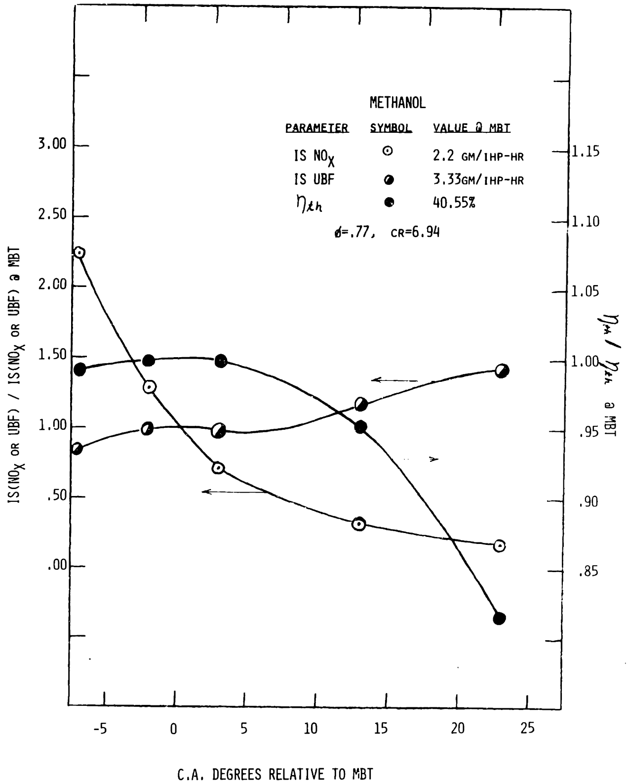
Figure 28 \eta_{th} , IS NO x emissions, and IS UBF emissions vs. spark advance relative to MBT for methanol
