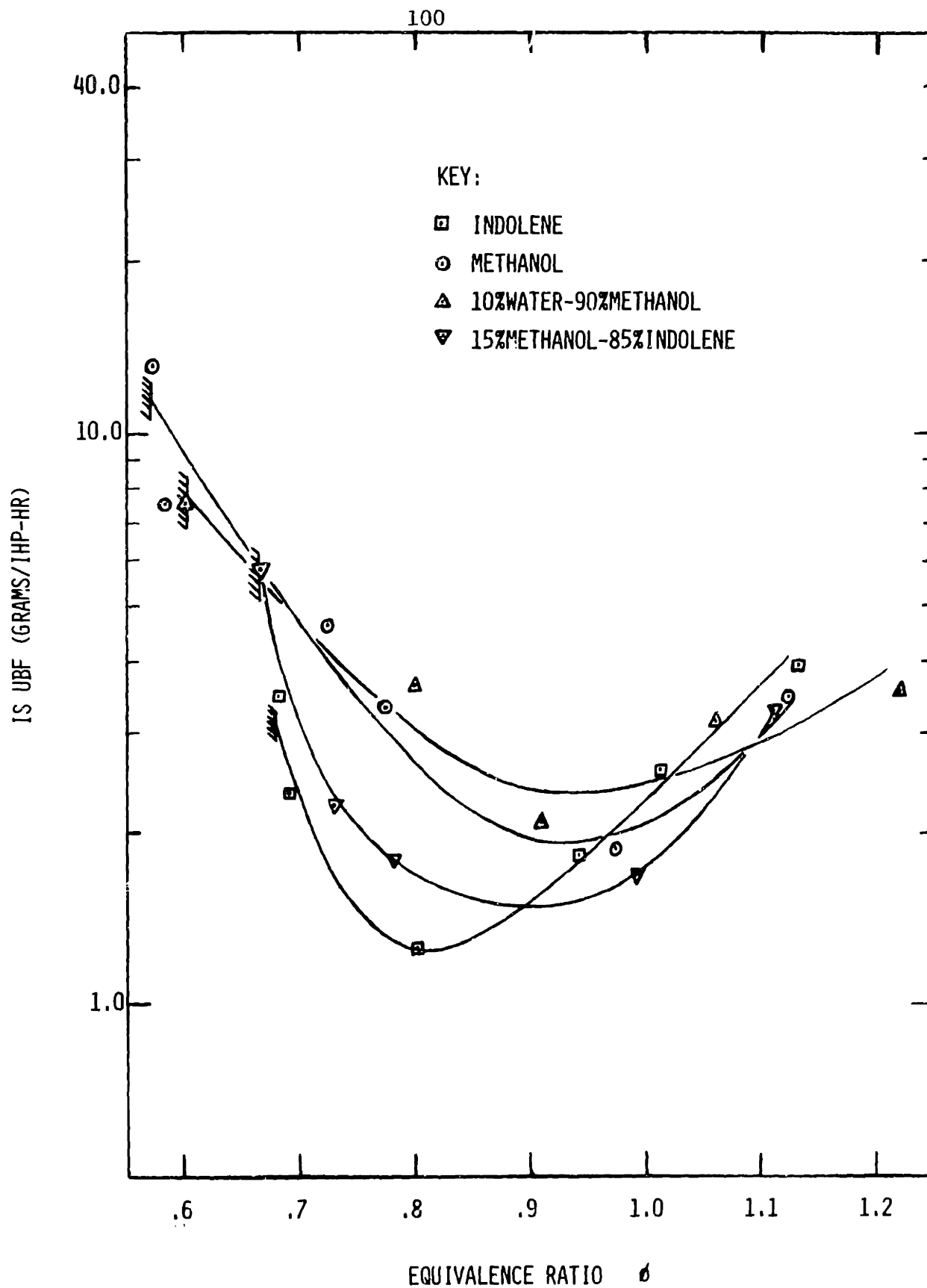
Figure 24 Indicated specific unburned fuel emissions (IS UBF) vs. equivalence ratio ( \phi ) and fuel type at baseline conditions (Table 4)
