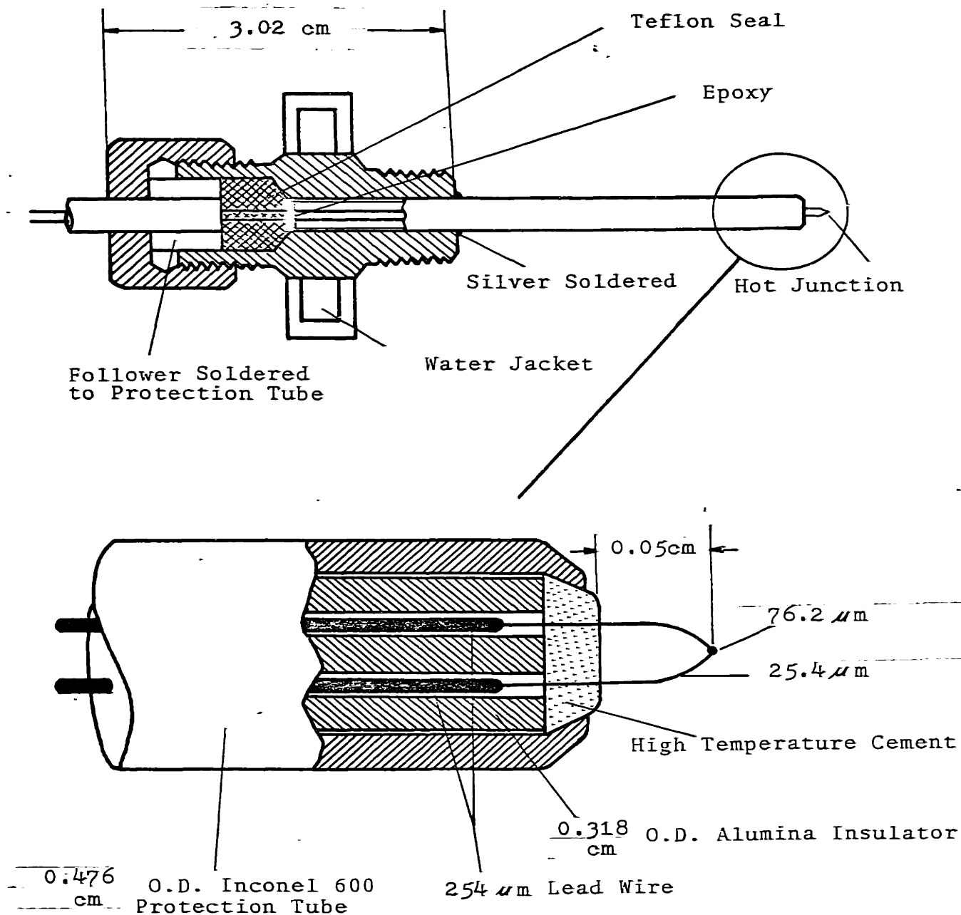
Fig. III-1 Thermocouple probe assembly Drawing not to Scale
