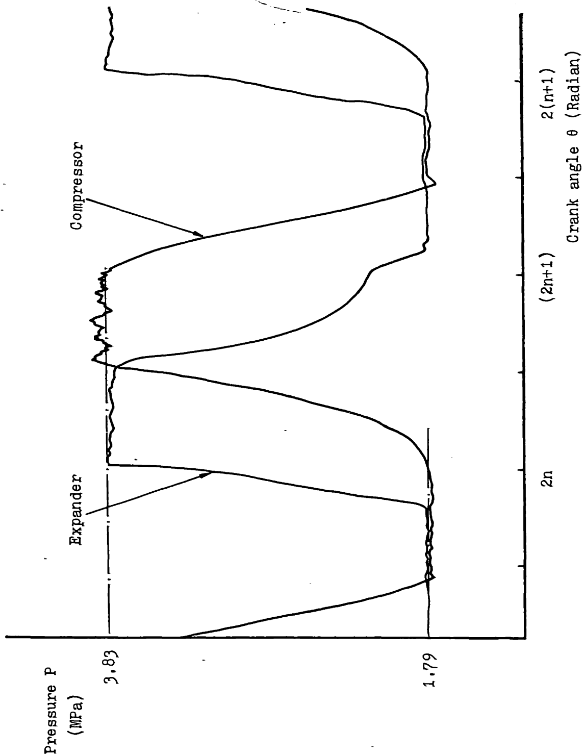
Fig. A-6 P-θ diagram for expander and compressor - Test #3
