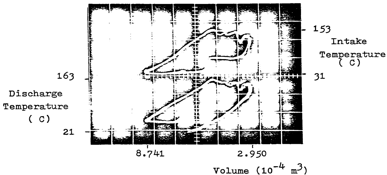
(a) Compressor Discharge and Intake
