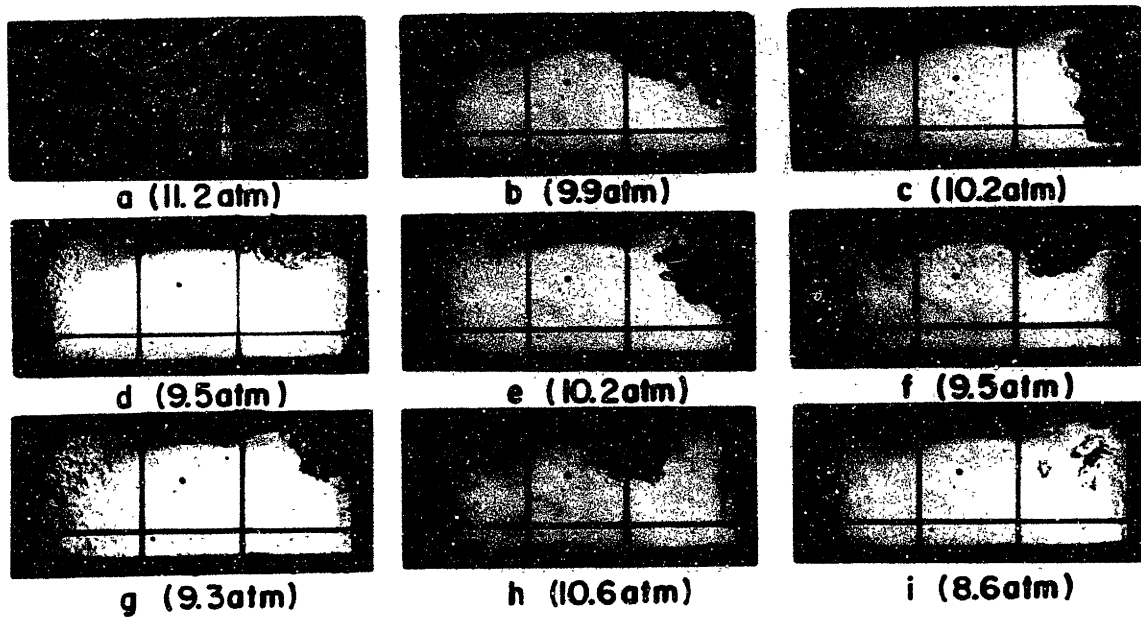
Fig 4.10 - Still pictures taken 31° after spark (i.e. 24° BTC) from nine different cycles showing the variation in size, shape and the location of the flame from cycle to cycle. The detachment of the flame from the spark plug in h and i is due to the rotational motion shown in Fig 3.4.
