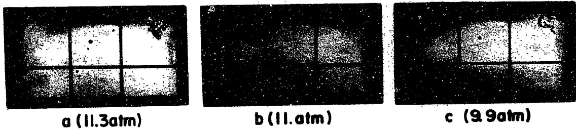
Fig 4.9 - Photographs taken at 14° after the spark of three cycles.
