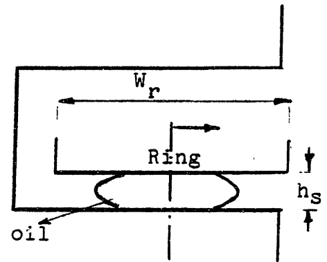
Fig A6.1.2 Schematic of squeezed oil flow
