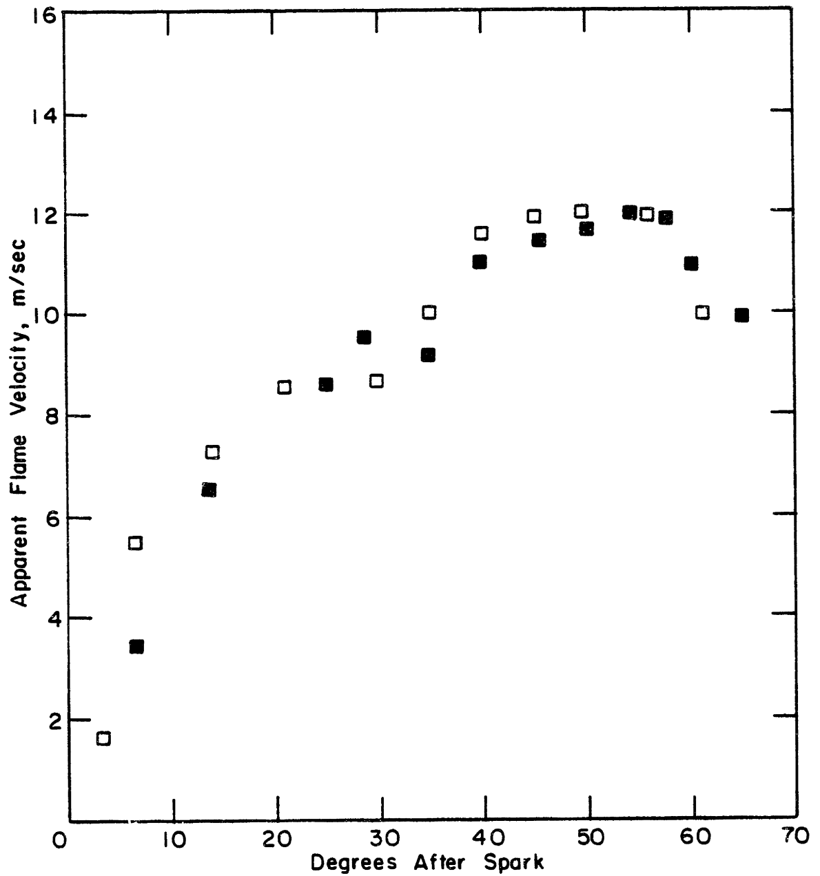
Fig 4.1 - Apparent flame velocity, average rate of flame travel normal to the flame front in the lab coordinates for two consecutive cycles.
