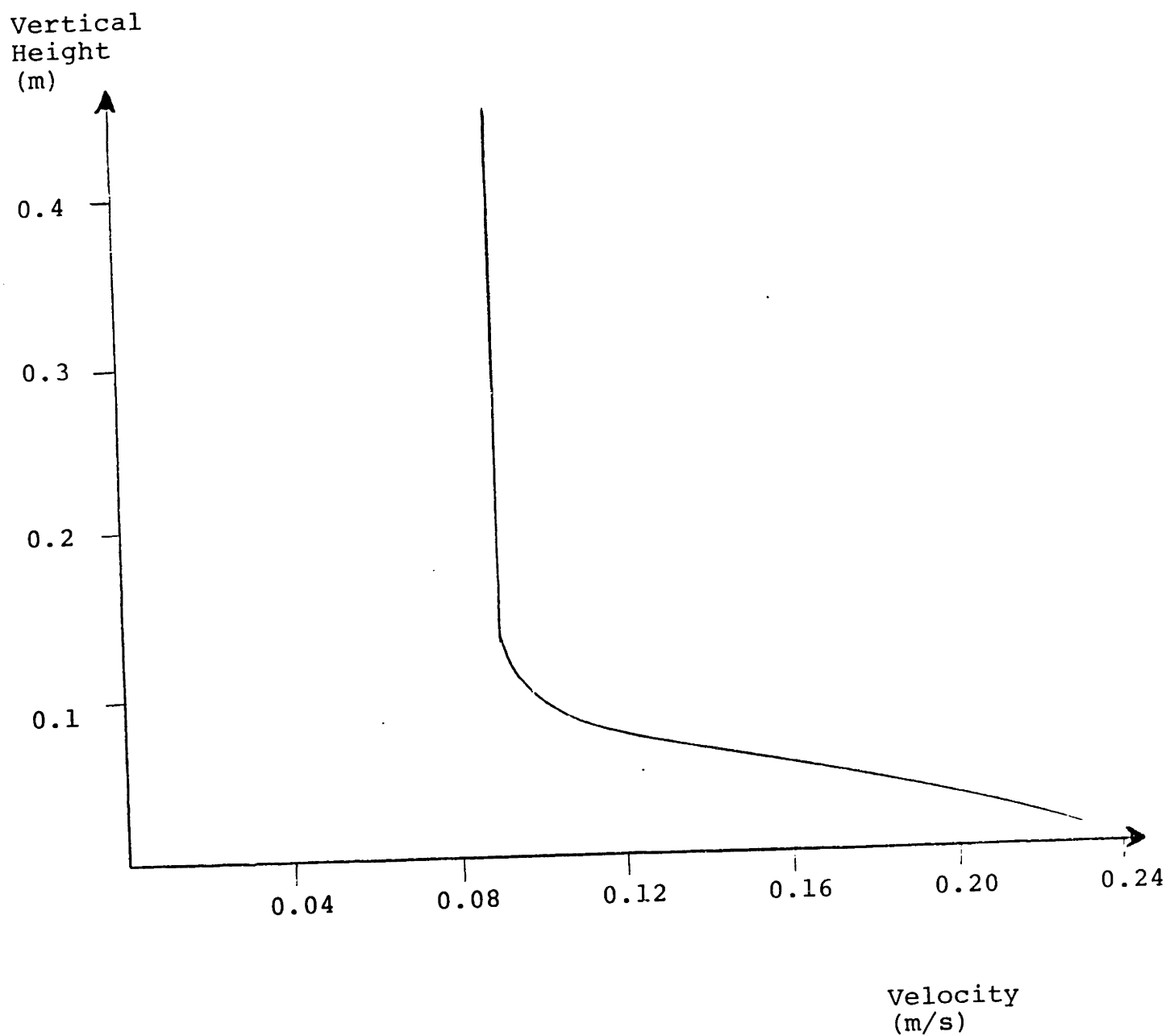
FIGURE 7: Jet Type Profile (Calculated from Hydrogen Bubble Flow Visualization)
