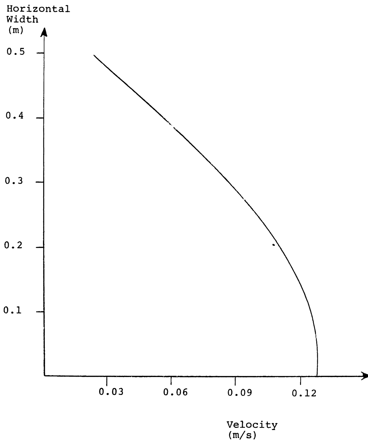
FIGURE 9: Left to Right Windshear Profile (Calculated from Hydrogen Bubble Flow Visualization)
