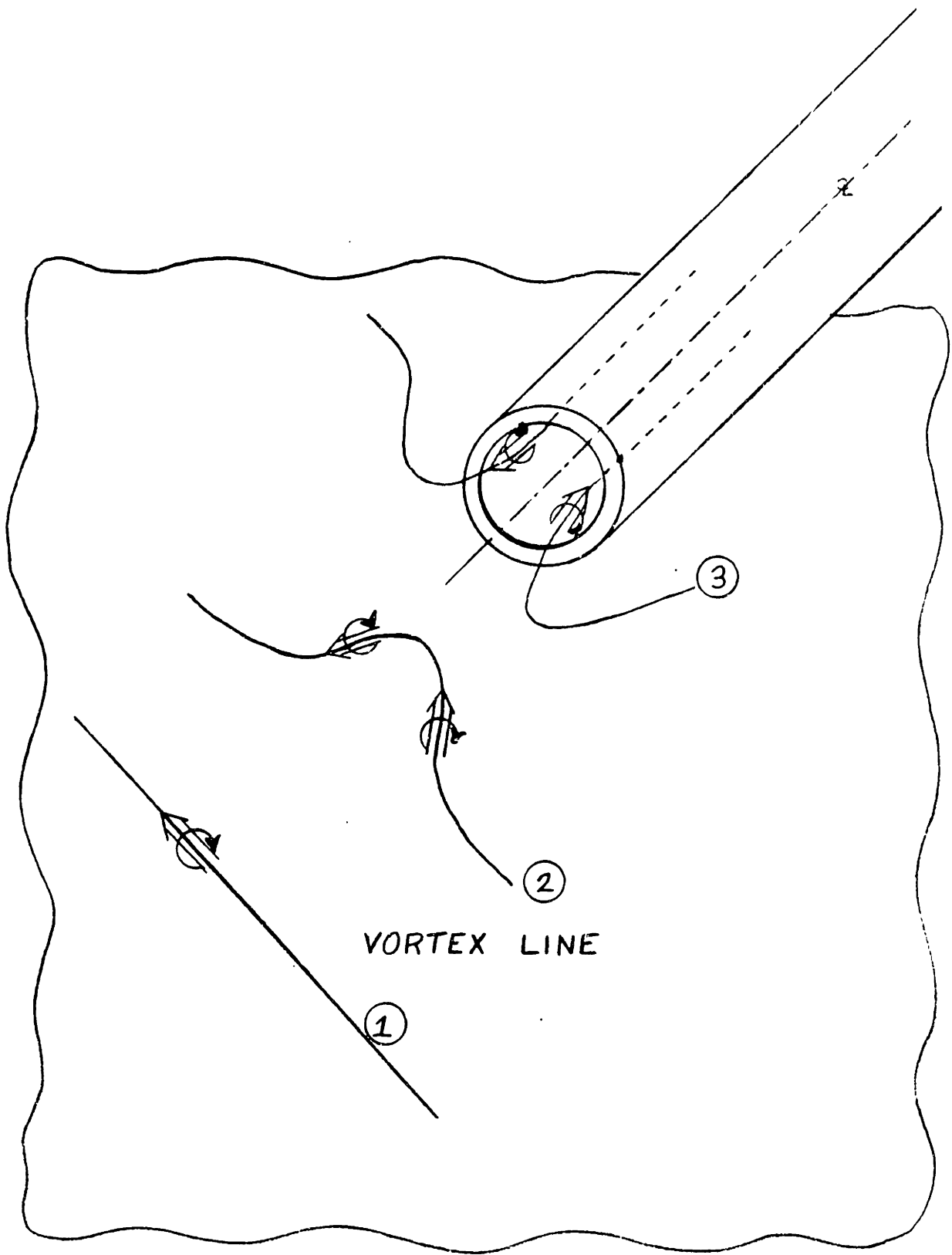
FIGURE 1: Suggested Sketch of a Vortex Line at Three Instants of Time
