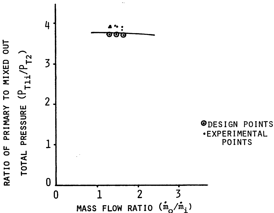
FIGURE 16. COMPARISON OF DESIGN AND MODELLING RESULTS TO EXPERIMENTAL MEASUREMENTS FOR P_{T1i}/P_{T2} VS \dot{m}_o/\dot{m}_i
