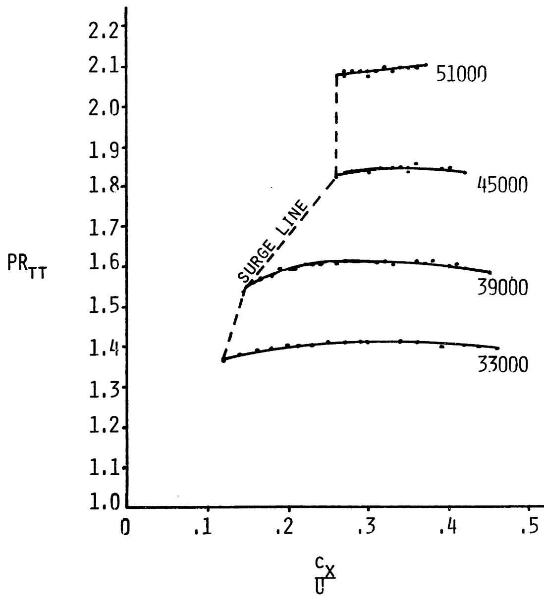
FIGURE 19. OVERALL COMPRESSOR CHARACTERISTIC
