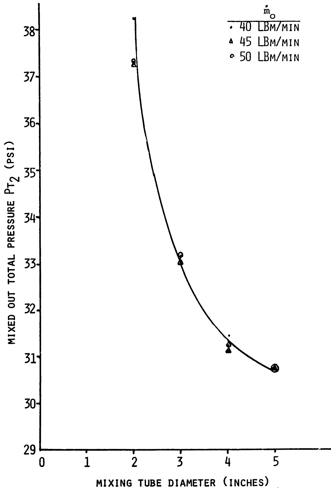
FIGURE 5. AIR EJECTOR RESULTS FOR P_{T1} = 125 PSI
