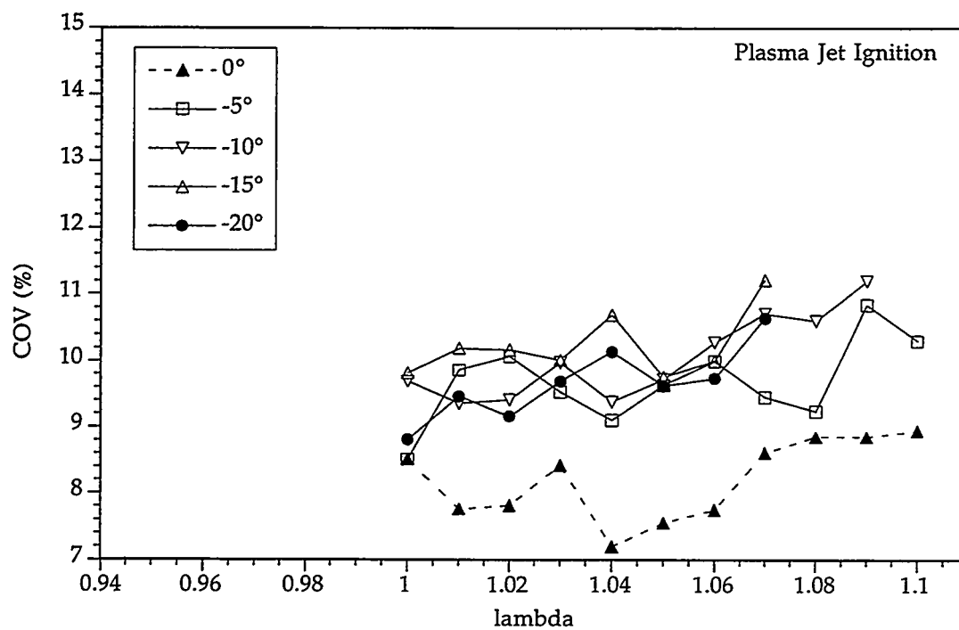
Figure 9.7: Comparison of COV of IMEP versus Lambda
