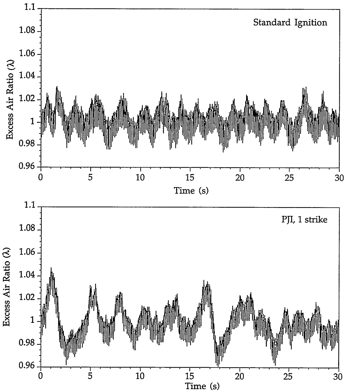
Figure 5.3: Comparison of UEGO Sensor \lambda Waveforms During Closed-Loop Stoichiometric Operation
