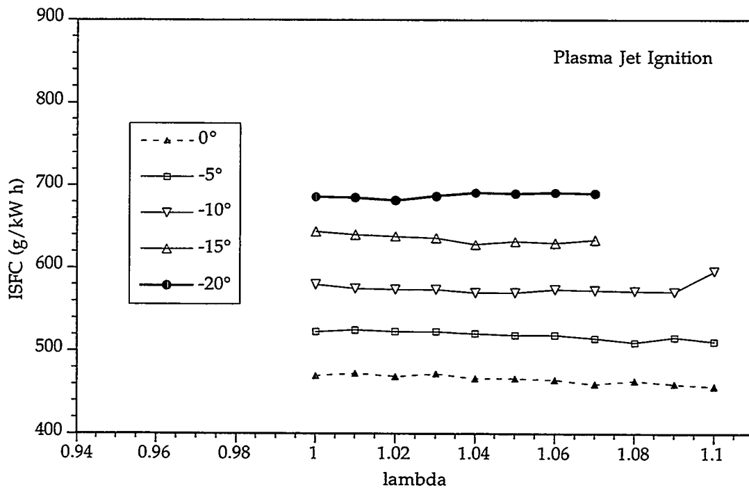
Figure 9.5: Comparison of Indicated Specific Fuel Consumption versus Lambda
