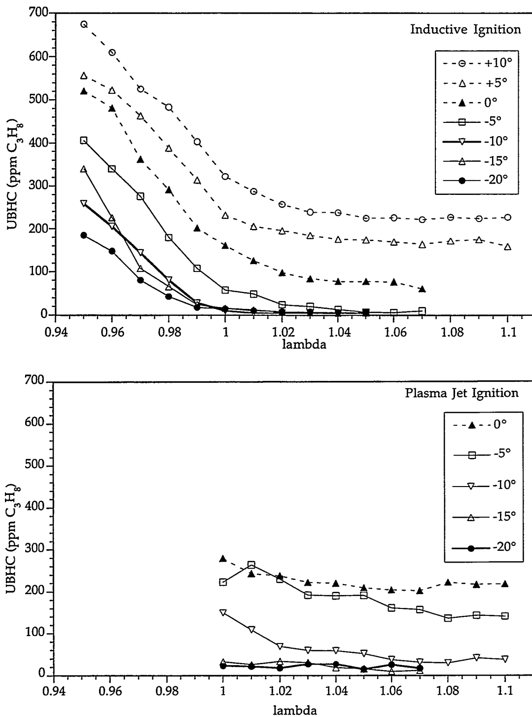
Figure 9.1: Comparison of Exhaust Hydrocarbon Concentration versus Lambda
