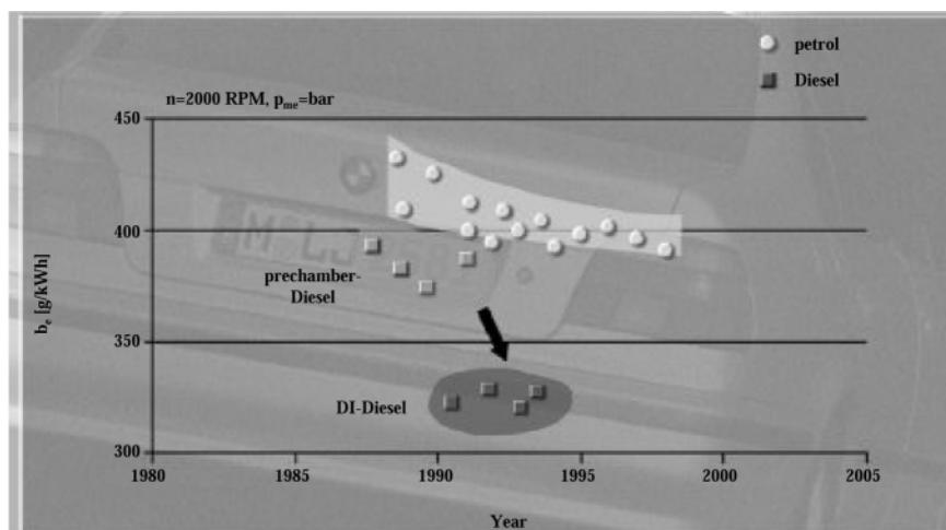
Figure 1. Trend in specific fuel consumption
