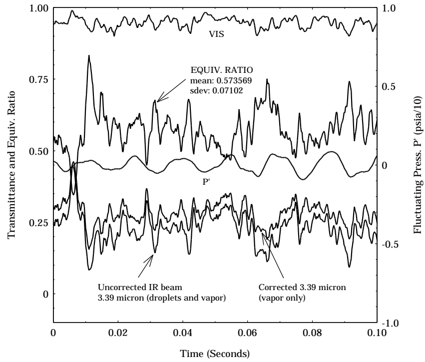
Figure 3: Time-resolved FAR measurements at 4.42 atm, 616 K, approx. 2.7 cm pathlength, \text{FAR}_{\text{METER}} = 0.039 ( \Phi=0.57 ).
