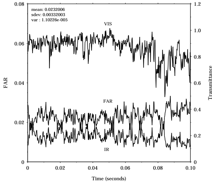
Figure 5: Time-resolved measurements at 14.9 atm, 755 K, FAR_{METER} = 0.022 ( \Phi=0.32 ).
