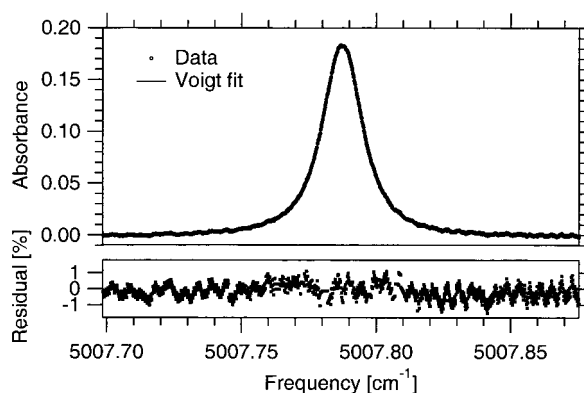
Fig. 5. Sample line shape for static-cell measurements of CO 2 absorbance at 5007.787 \text{cm}^{-1} for the R(50) transition with P = 68.1 Torr, L = 40 cm, and T = 294 K.
