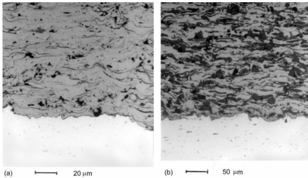
Figure 3. Typical internal coating sprayed on AlSi cast alloy. (a) Low alloyed carbon steel with built solid lubricant ( HV_{0.3}=400 ) (b) Composite metal ceramic ( HV_{0.3}=530 )
