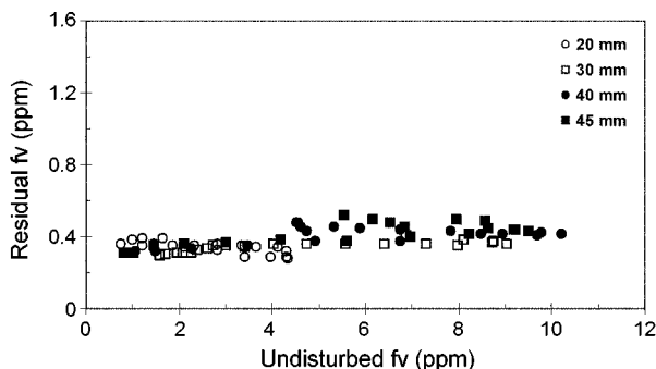
Figure 6. Undisturbed and residual soot volume fractions over the various flame heights.
