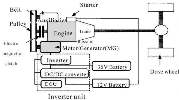
Figure 2. System configuration.
