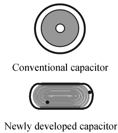
Figure 5. The shape of the capacitor (horizontal cross-section).
