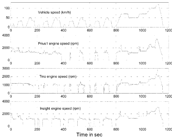
Figure 3. Vehicle and i.c. engine speeds during an NMVEG cycle.
