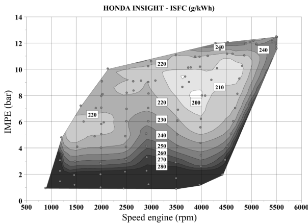
Figure 10. Measured insight indicated consumption maps according to engine speed and IMPE.
