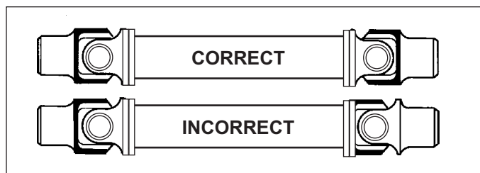
Proper U-joint alignment
